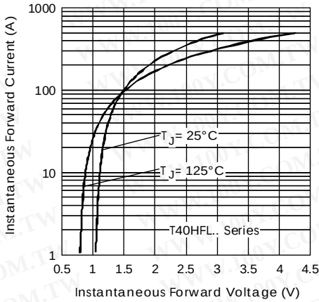
Fig. 46 - Forward Voltage Drop Characteristics
