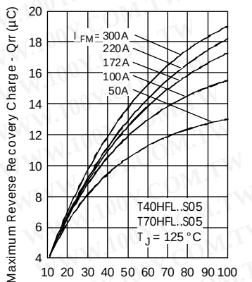
Fig. 23 - Recovery Charge Characteristics
