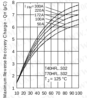
Fig. 20 - Recovery Charge Characteristics
