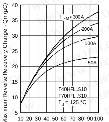
Fig. 26 - Recovery Charge Characteristics
